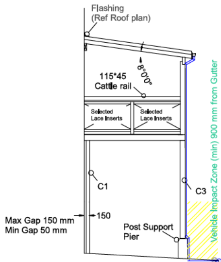
North-East Elevation
