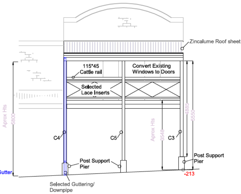
North-West (Main st) Elevation
